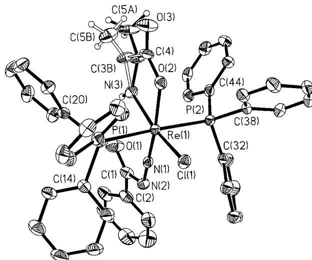
Figure 5. An ORTEP-3 representation of 5 . Ph hydrogen atoms and solvent molecules have been omitted for clarity.
