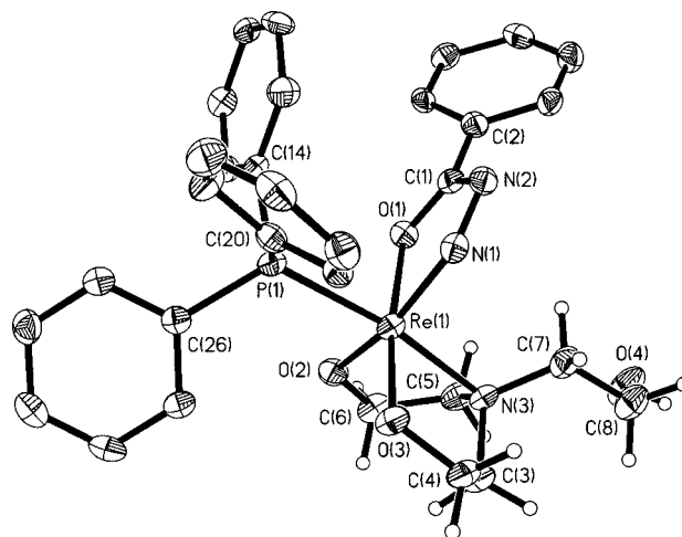
Figure 2. An ORTEP-3 representation of 2 . Ph hydrogen atoms have been omitted for clarity.
