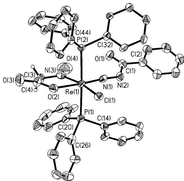
Figure 4. An ORTEP-3 representation of 4 . Ph hydrogen atoms have been omitted for clarity.
