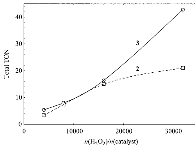
Figure 7. Effect of the oxidant-to-catalyst molar ratio on the total TON values in the oxidation of cyclohexane catalyzed by complexes 2 and 3 .
