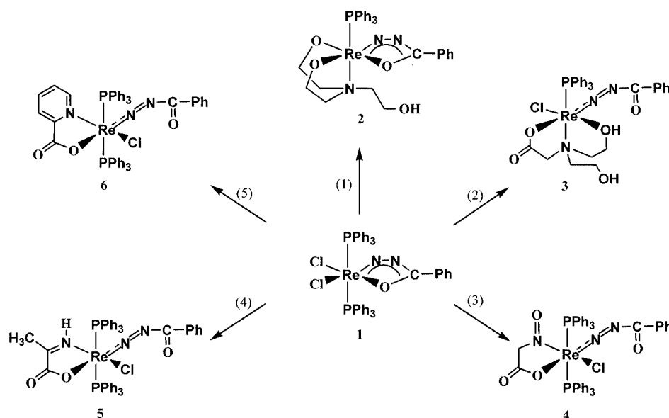
Scheme 1. (1) \text{N}(\text{CH}_2\text{CH}_2\text{OH})_3 ; (2) \text{N}(\text{CH}_2\text{CH}_2\text{OH})_2(\text{CH}_2\text{COOH}) (bicine); (3) \text{HON}(\text{CH}_2\text{COOH})_2 (HIDA); (4) \text{HON}\{\text{CH}(\text{CH}_3)\text{COOH}\}_2 (HIDPA); (5) \text{NC}_5\text{H}_4\text{COOH}-2 .
