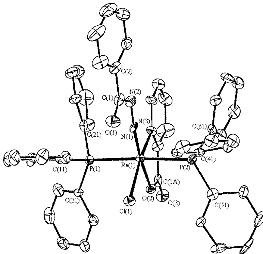
Figure 6. An ORTEP-3 representation of 6 . Hydrogen atoms and solvent molecule have been omitted for clarity.
