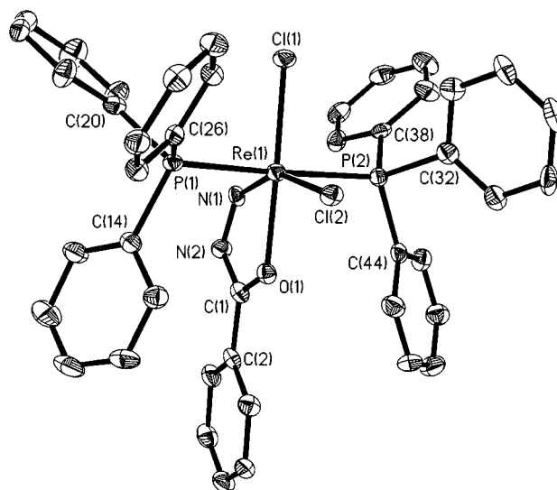
Figure 1. An ORTEP-3 representation of 1 . Hydrogen atoms and solvent molecule have been omitted for clarity.
