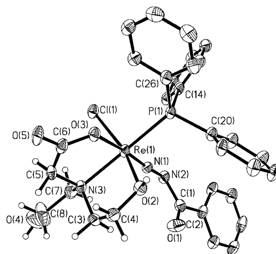
Figure 3. An ORTEP-3 representation of 3 . Ph hydrogen atoms and solvent molecules have been omitted for clarity.
